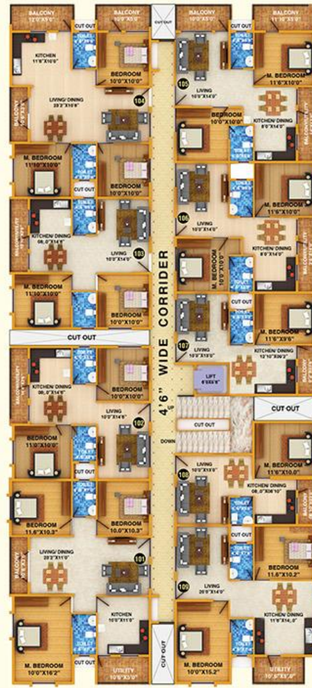
A,B,C,D & E - BLOCK TYPICAL FLOOR
