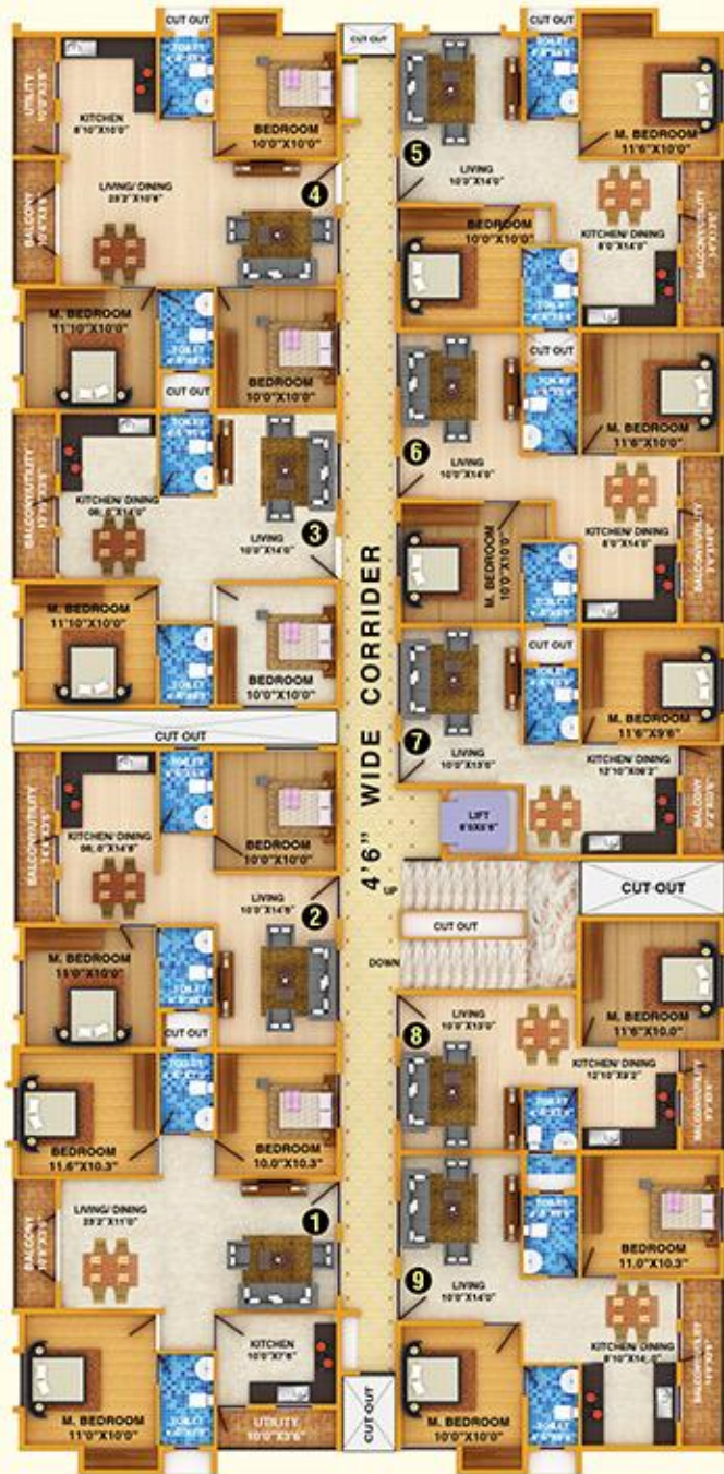
A,B,C,D & E - BLOCK GROUND FLOOR
